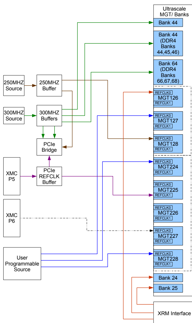
Figure 5 : Clocks
