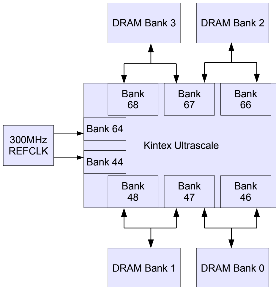
Figure 8 : DRAM Banks
